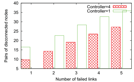
Fig. 5. Affected node pairs in split architecture (one controller)
